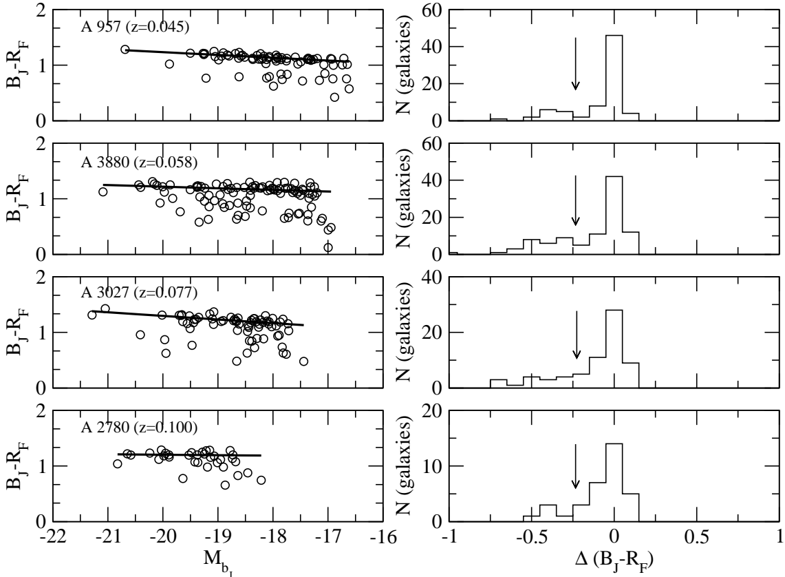
Figure 1. Colour-magnitude relation (left) and histogram (right) of marginalised colour distribution (opposite each colour-magnitude relation) for four representative clusters. The arrow in the histogram indicates the blue/red separation (see text)
