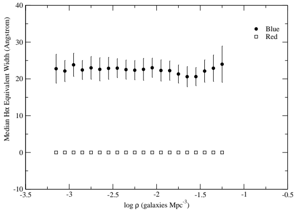
Figure 6. Median H \alpha equivalent widths (in Angstroms) for blue and red galaxies in the field as a function of density. Errors are interquartile means. The errors for the red galaxies are smaller than the symbols.
